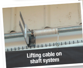
Transmission shaft system
